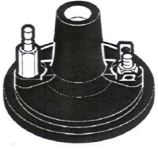
09-204 12 Volt Ballast Coil for use on a ballast system where a resistor or resistance wire is used. Can diameter 55mm.
